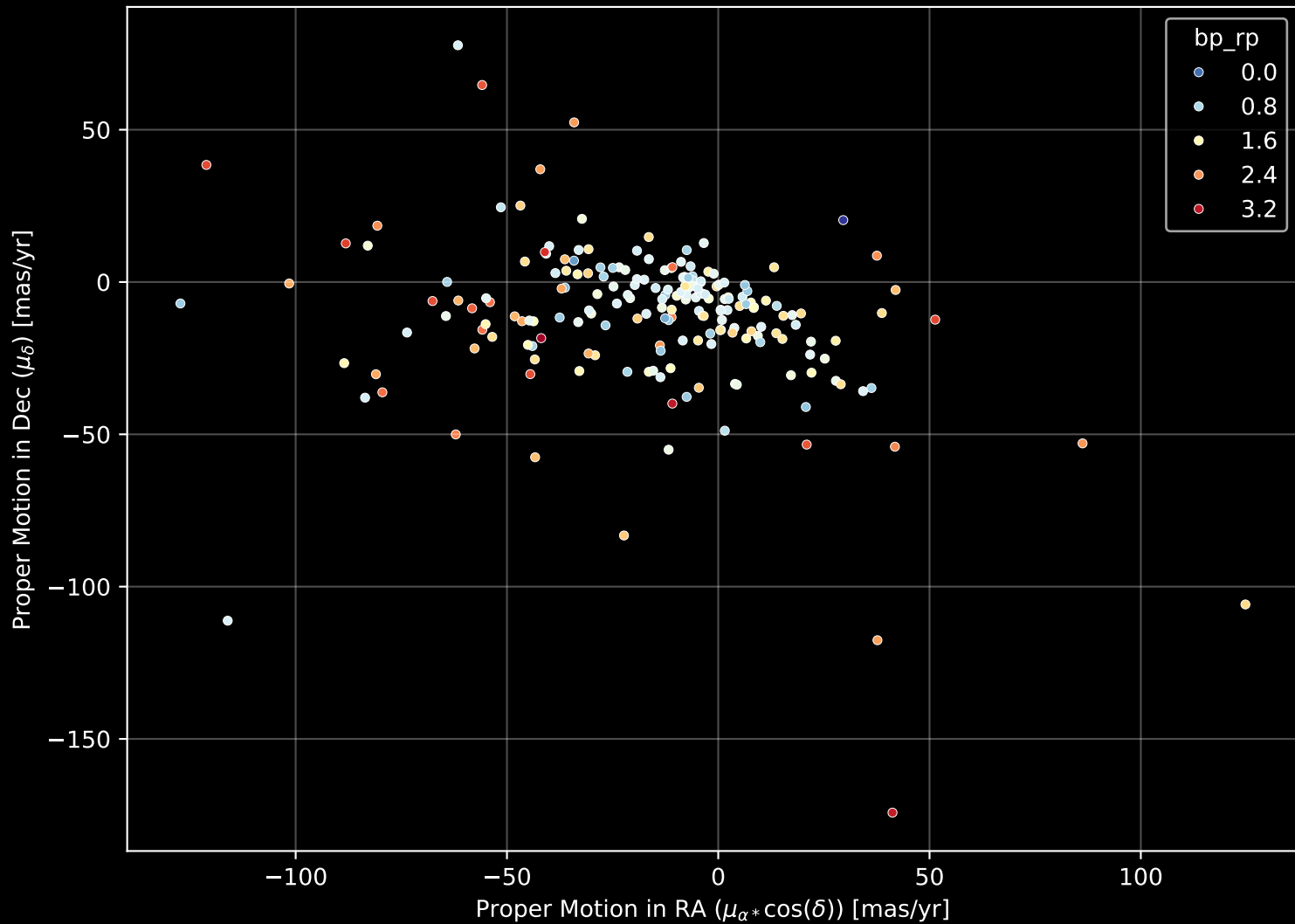
APOGEE DR17 Field: [K2_C1_264+52_btx] Proper Motion Diagram (n= 201)
