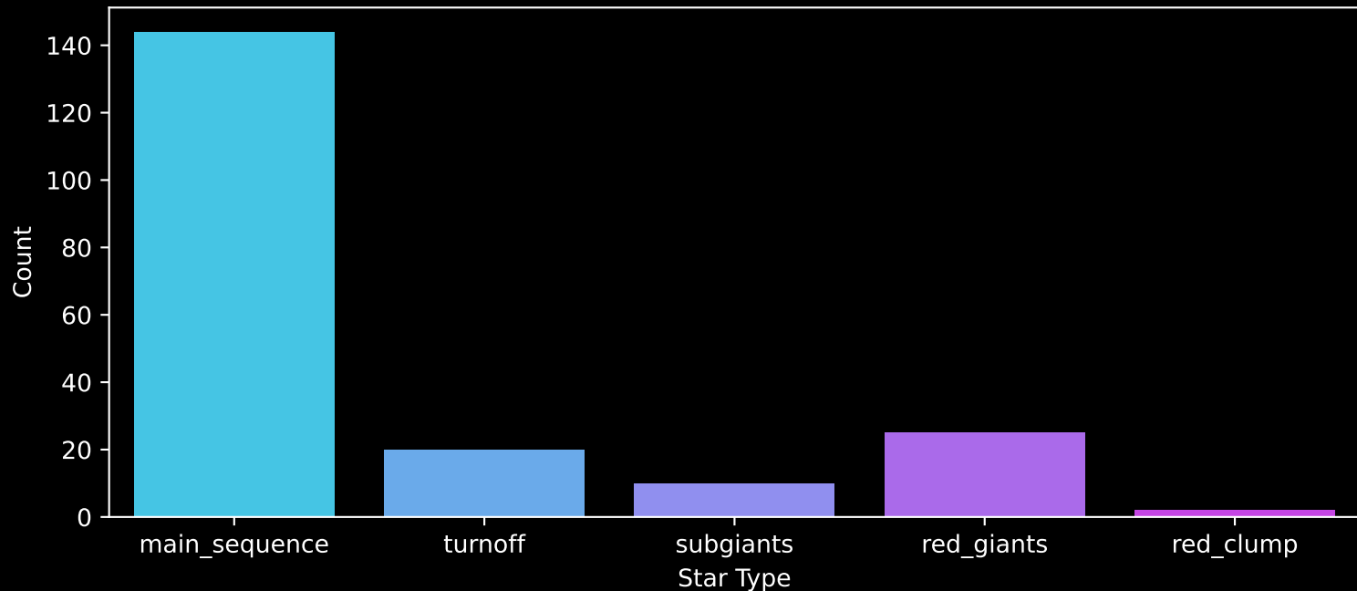
APOGEE DR17 Field: [K2_C1_264+52_btx] Count plot of Star Type
