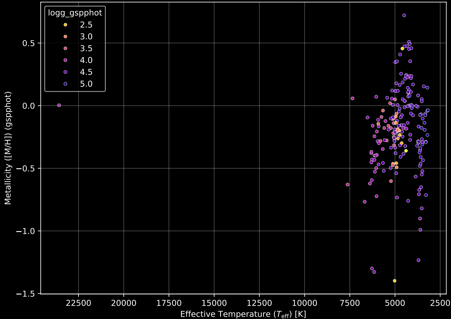
APOGEE DR17 Field: [K2_C1_264+52_btx] Stellar Population Parameters (n= 201)
