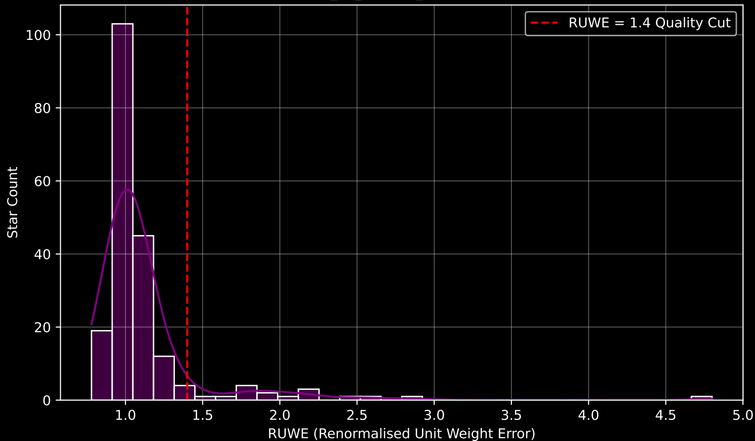
GAPOGEE DR17 Field [K2_C1_264+52_btx] RUWE Distribution (n= 199)
