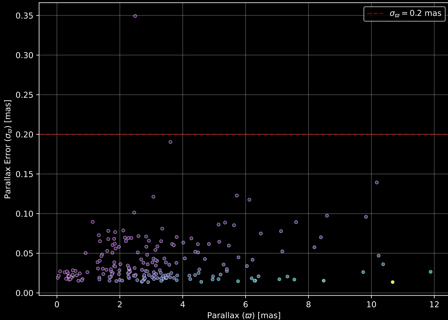
APOGEE DR17 Field: [K2_C1_264+52_btx] Parallax Quality (n= 201)
