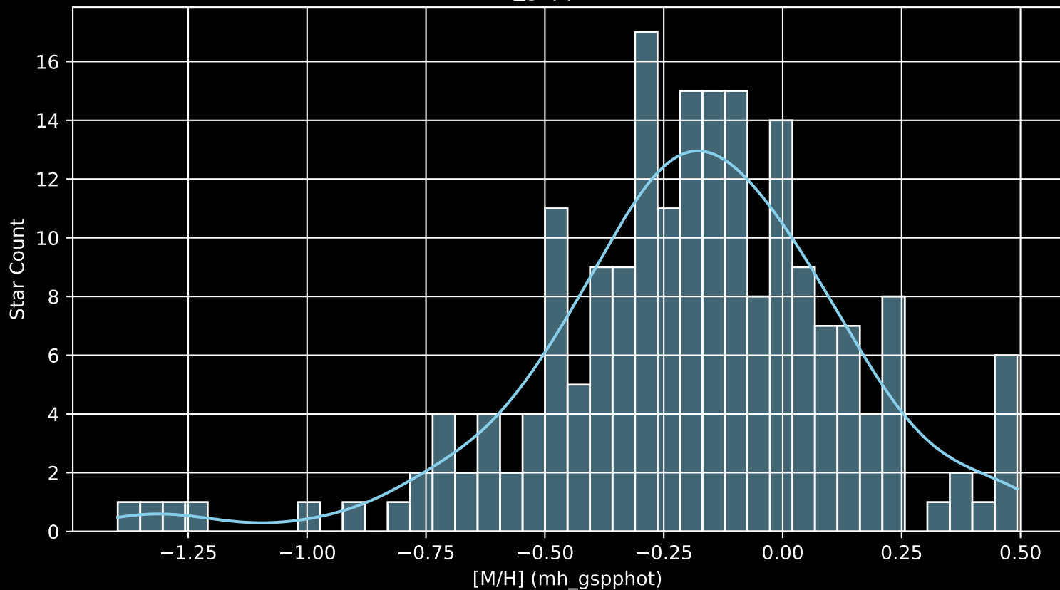
APOGEE DR17 Field: [K2_C1_264+52_btx [M/H] (mh_gspphot) (n= 199)
