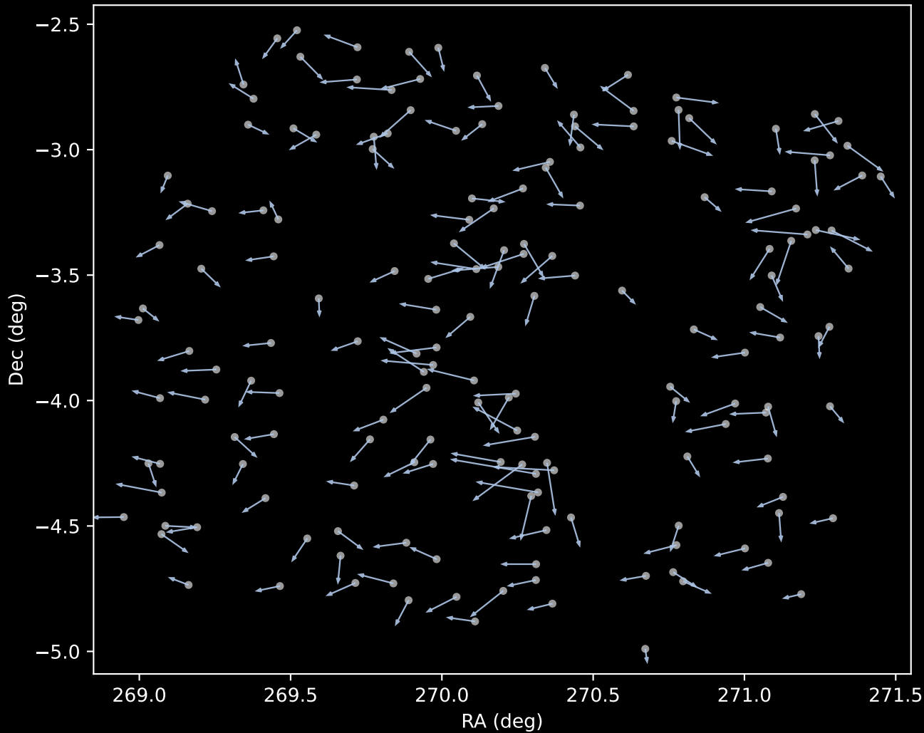
APOGEE DR17 Cluster 1 Proper Motion Vectors (n=171)
